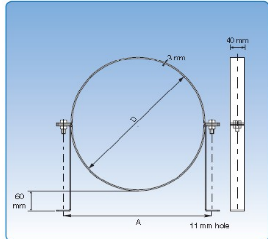
Diameter: 315-800mm
