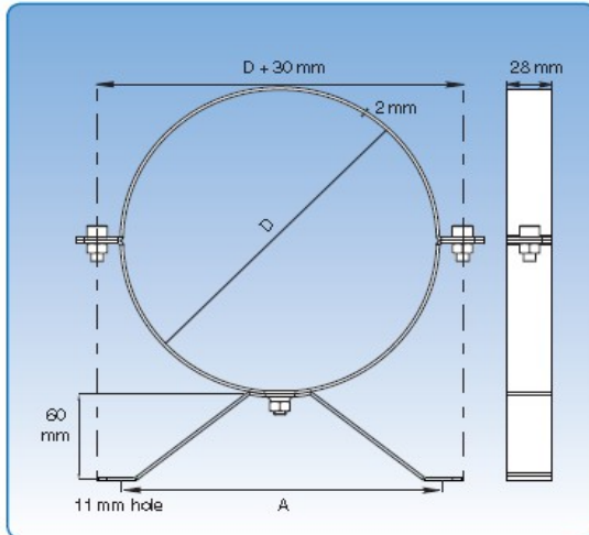
Diameter: 80-300mm
